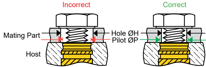
The hole in mating part must be smaller than the Insert pilot diameter in the host to prevent the Insert from pulling through the assembly - known as "Jack-Out"
